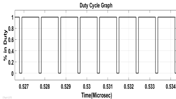
Fig -7: Duty cycle graph at an irradiance of 500 watt/meter square
