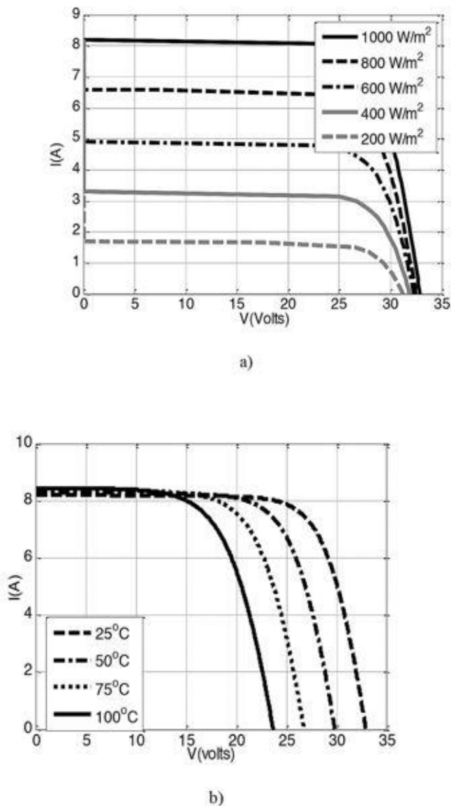
Fig -1 : (a) I-V characteristics of PV panel for different irradiance level. (b) I-V characteristics corresponding to different temperature.
