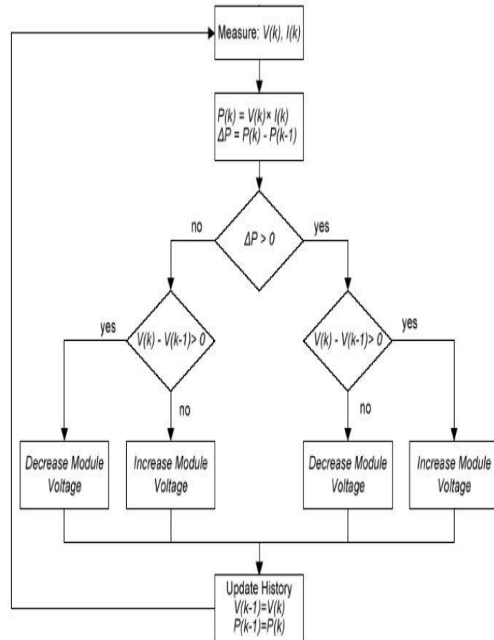
Fig -2: The flowchart of P and O algorithm for tracking maximum power from PV panel
