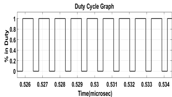
Fig -6: Duty cycle graph at an irradiance of 1200 watt/meter square
