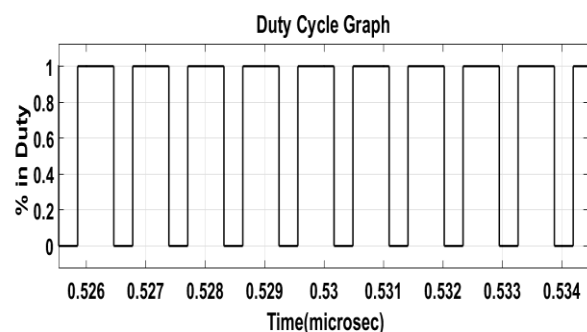
Fig -6: Duty cycle graph at an irradiance of 1200 watt/meter square
